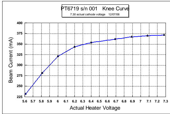
Figure6. Fast warm cathode knee curve - TMD
