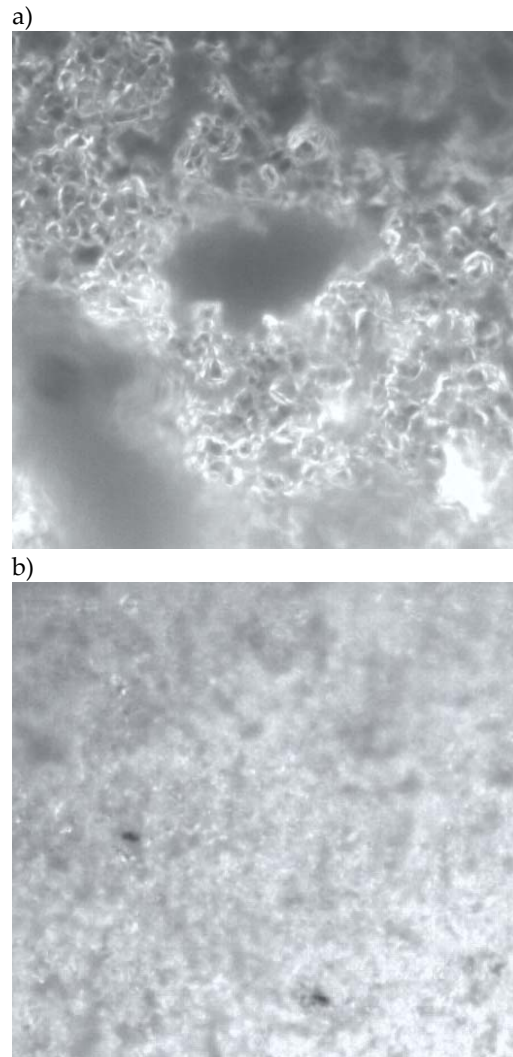
Figure4. Sintered ceramic potting a) Mix 15,1800C, x30obj, porous structure, b) Mix 19, 1850C, x50obj, modified mixture
