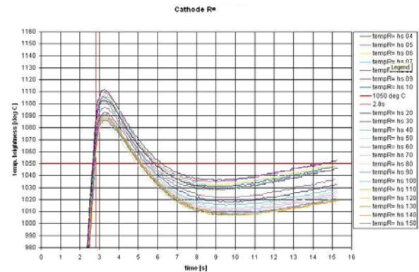
Figure7. Cathodes brightness temperatures on fast warm up tests a) 4.5s and 3.5s cycle, b) 2.8s cycle
