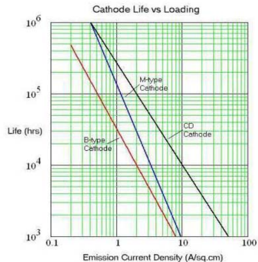
Figure3. Cathode life as a function of cathode loading
