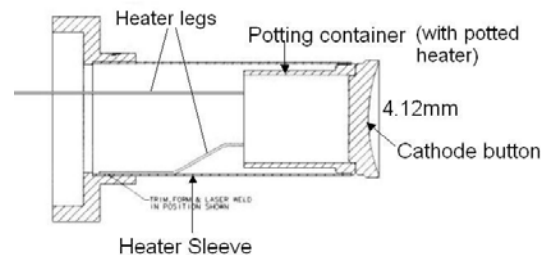
Figure1. TMD fast warm cathode
