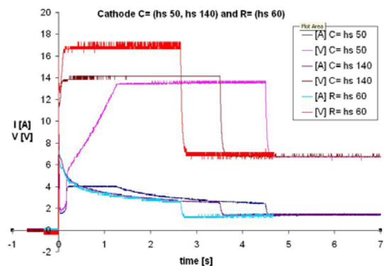
Figure5. Voltages and currents for 4.5s, 3.5, and 2.8s fast warm up times
