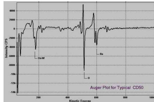
Figure2. Auger plot for typical CD cathode surface
